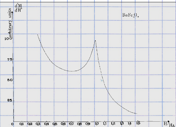
FIG. 5. Experimental plot of d^2M/dH^2 vs H = H_{\text{ext}} - NM for an isotropic polycrystalline sample of \text{BaFe}_{12}\text{O}_{19} . H_{\text{ext}} is the applied field, and N denotes the demagnetizing factor of the sample.
